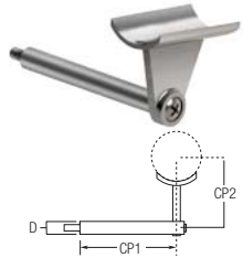
49-308PM/1H Post-mounted Handrail Bracket Tube: 1.5"* CP1: 2.25" CP2: 2.125" D: 0.47"
