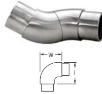
49-731A/424 Adjustable Radius Ell W: 2.76" L: 2.76"
