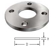
49-541/424 Floor Flange D: 3.94" H: 0.32"
