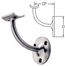
49-301/424 Handrail Bracket CP: 2.5" D: 2.56"
