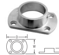
49-511/424 Cut Wall Flange D: 3.35" W: 2.12" H: 1.0"
