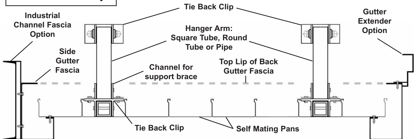
Architectural Canopy: Front View Assembly
